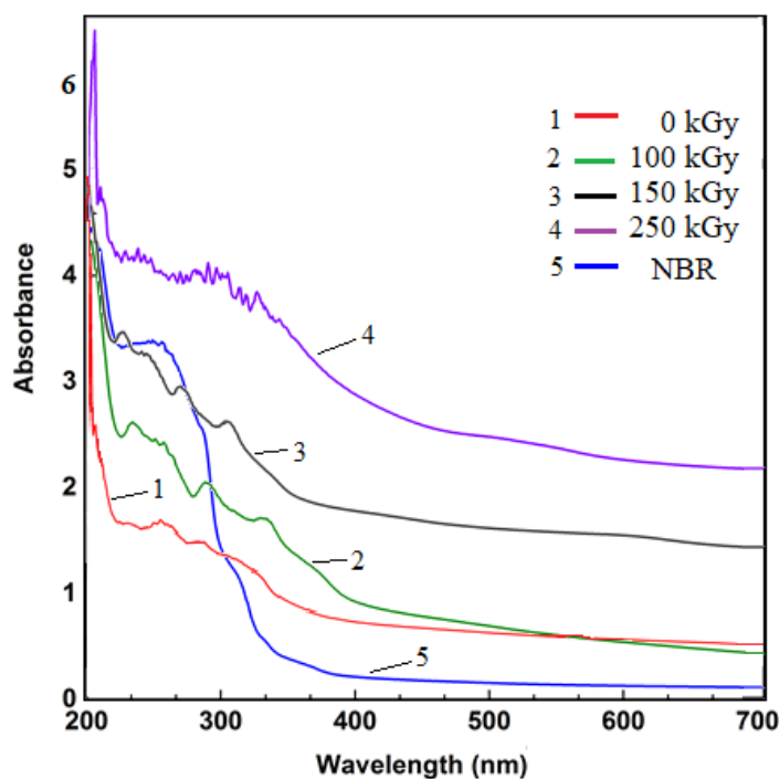
Fig. 4. UV-Vis spectrum of NBR and NBR / ZrO_2 / DSCB nanocomposite obtained by gamma radiation
