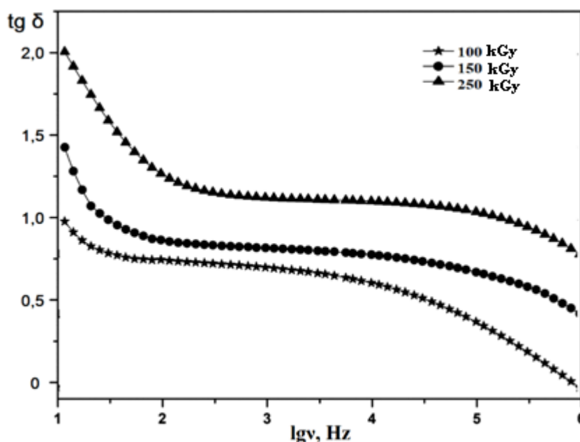
Fig. 3. Frequency dependence of the dielectric loss tangent of irradiated nanocomposites (NBR + DSCB + ZrO 2 )
