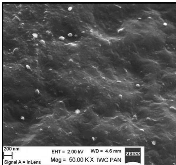
Fig. 5. SEM image of the surface of the NBR / ZrO 2 / DSCB nanocomposite lowed by gamma irradiation by a dose of 250 kGy.
