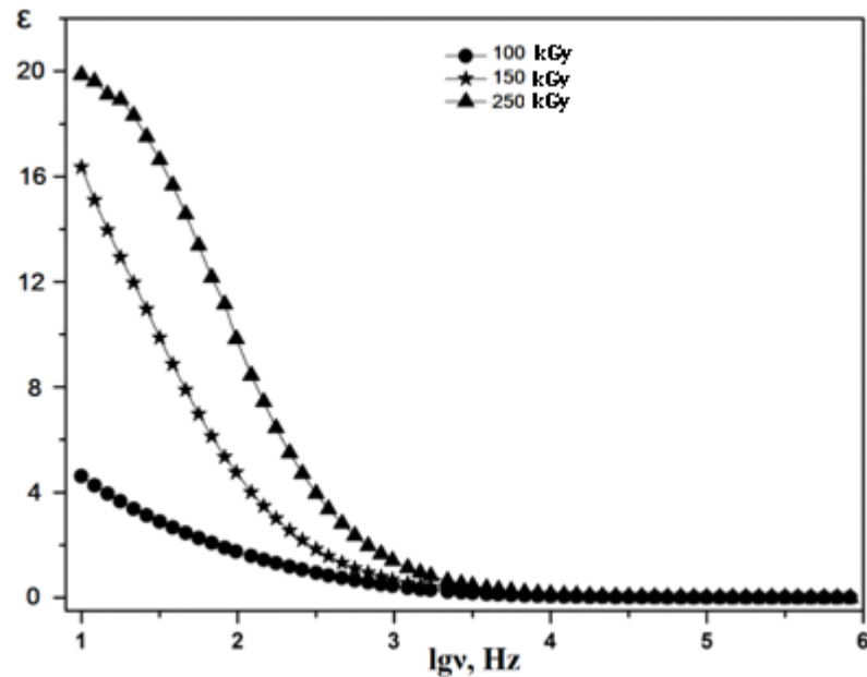
Fig. 2. Frequency dependence of the dielectric constant of irradiated nanocomposites (NBR + DSCB + ZrO 2 )
