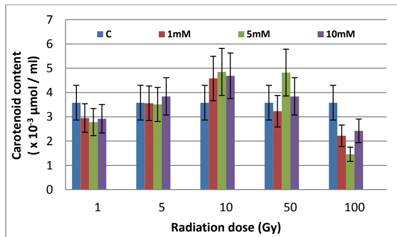
Fig. 4. Change dynamics of the carotenoids amount under dual stress condition.
