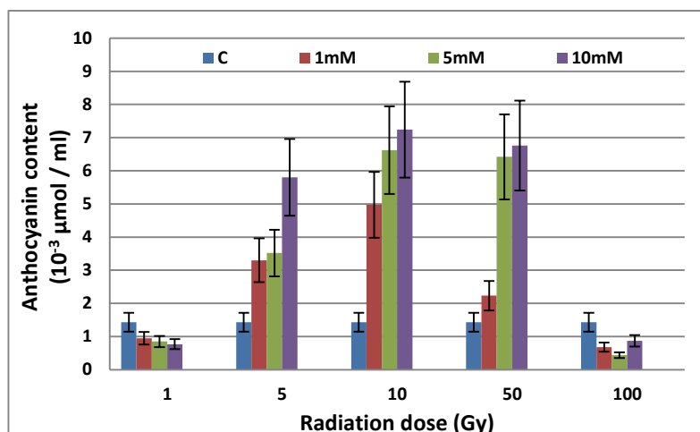
Fig. 5. Change dynamics of the anthocyanin amount under dual stress condition.
