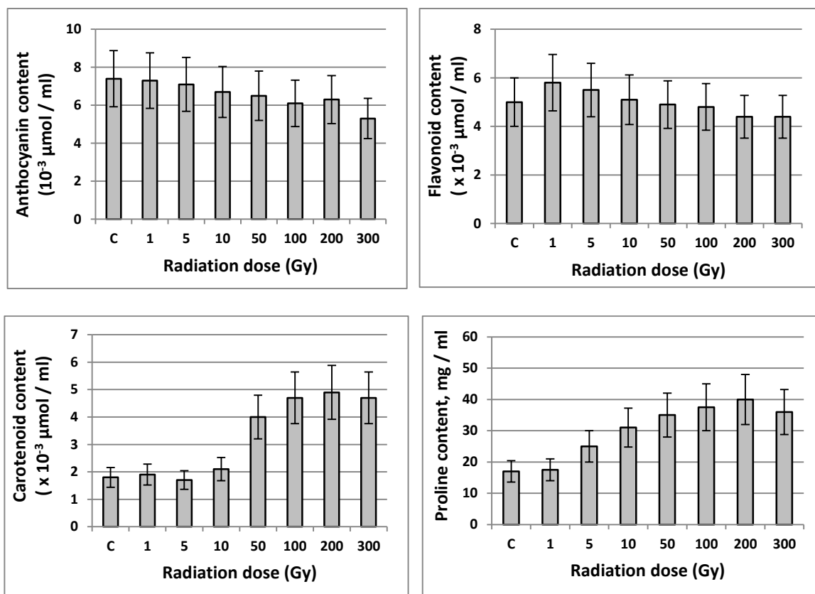
Fig. 2. Change dynamics of low-molecular antioxidants depending on the dose of seeds irradiation.
