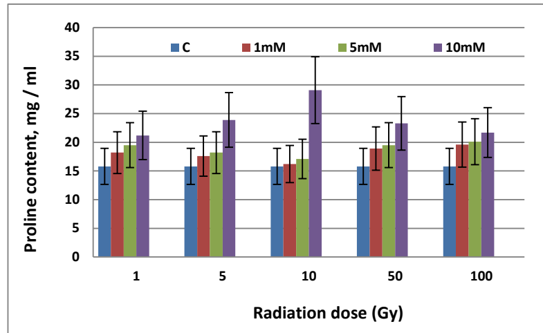
Fig. 3. Change dynamics of the proline amount under dual stress condition.
