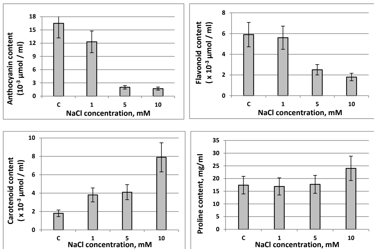
Fig. 1. Change dynamics of the amount of low-molecular antioxidants depending on NaCl concentration.
