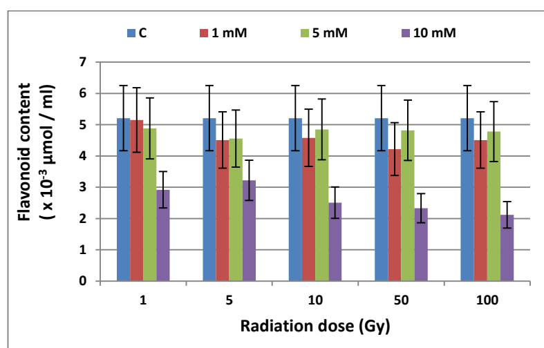
Fig. 6. Change dynamics of the number of flavonoids in dual stress conditions.
