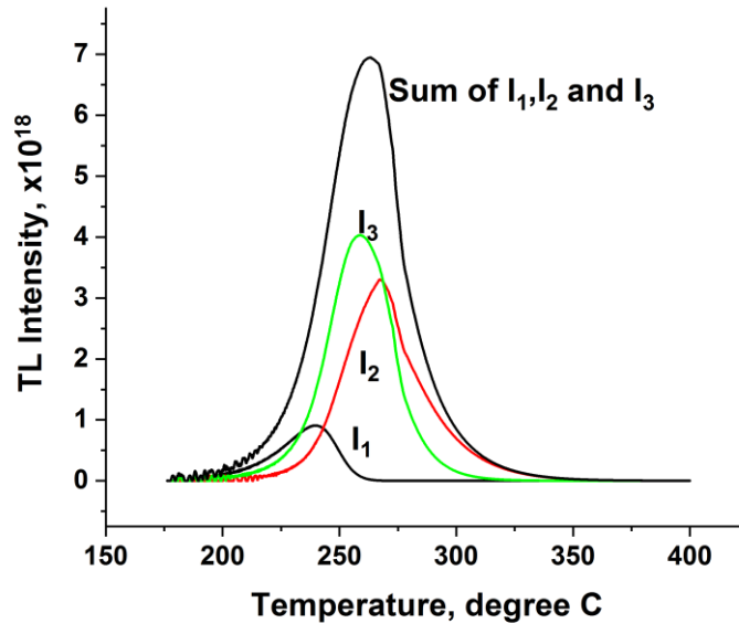
Fig. 4. Three TL peaks ( I_1 , I_2 , and I_3 ) as calculated with the model of three recombination centers and one trapping state. They might be attributed to three components in the emission of TL in quartz, namely, UV, blue, and green. The set of parameters applied is given in the text. The sum of peaks is attributed to the total TL peak.
