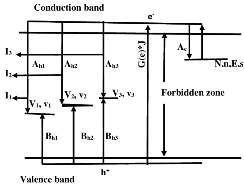
Fig. 1. One trap three recombination center model for the thermoluminescence process. The transitions take place during the irradiation and the heating of the sample is indicated by arrows. The meaning of the different parameters and the values chosen for them are given in the text.
