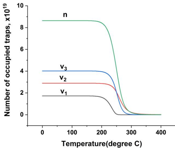
Fig. 3. Kinetics of accumulation of trapped holes and electrons during the heating stage. v_1 , v_2 , and v_3 are the concentrations trapped holes, and n stands for the trapped electrons.
