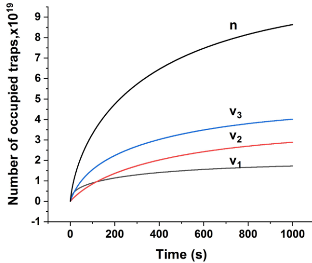
Fig. 2. Kinetics of accumulation of trapped holes and electrons during the irradiation stage. v_1 , v_2 , and v_3 are the concentrations trapped holes, and n stands for the trapped electrons.
