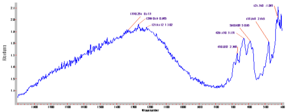
Fig. 1c. IR absorption spectrum of single crystal GaS after consequently 140 krad irradiation and annealing in vacuum ( 100^{\circ}\text{C} , 1 hour)
